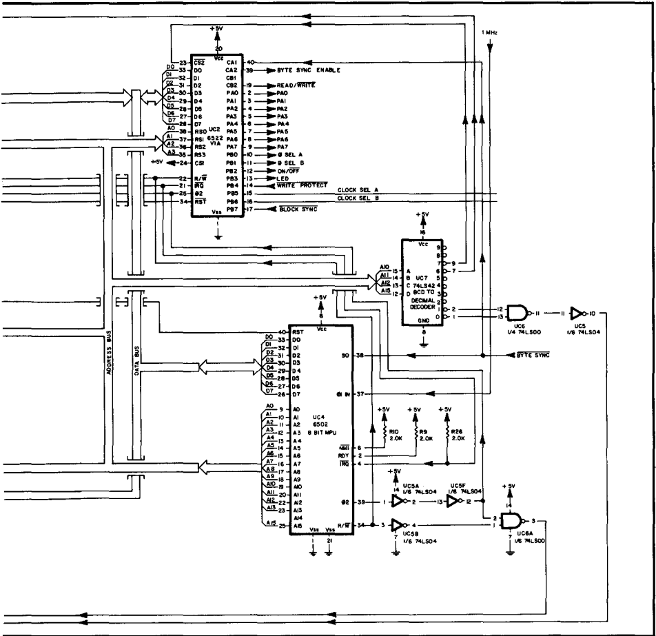
circuit, Model 1541.
